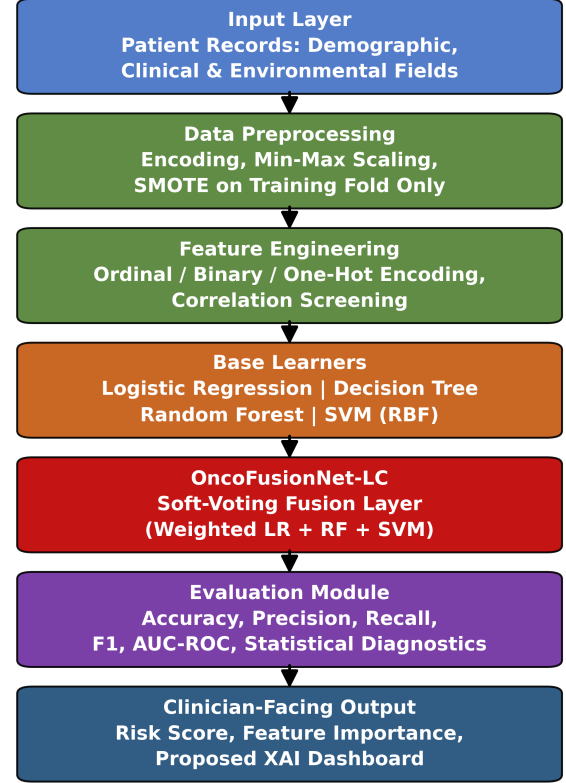
Fig. 1: Corrected end-to-end OncoFusionNet-LC pipeline.
