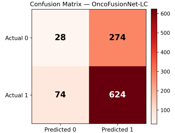
Fig. 5: Confusion matrix for OncoFusionNet-LC (test set, n = 1000 ).
