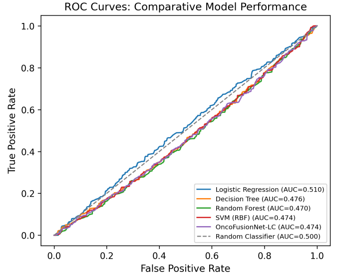
Fig. 4: ROC curves for all five models; every curve tracks the random-classifier diagonal.
